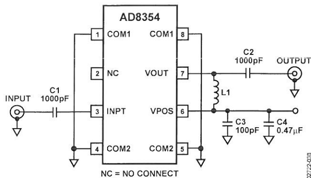
Figure 40. Evaluation Board Schematic
