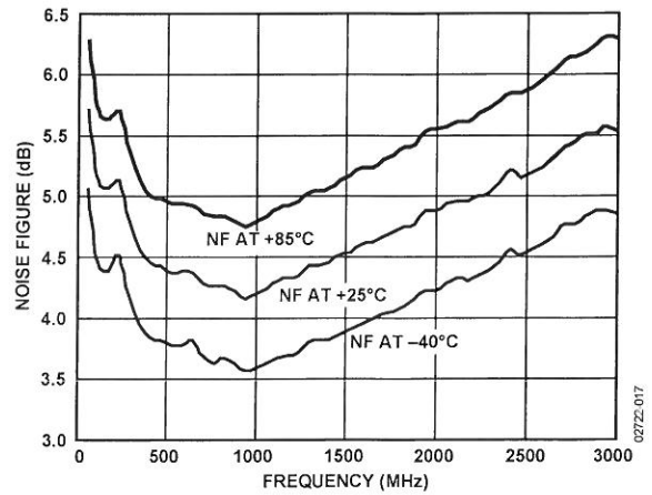
Figure 18. Noise Figure vs. Frequency, V_S = 3\text{ V}, T_A = -40^\circ\text{C}, +25^\circ\text{C}, \text{ and } +85^\circ\text{C}
