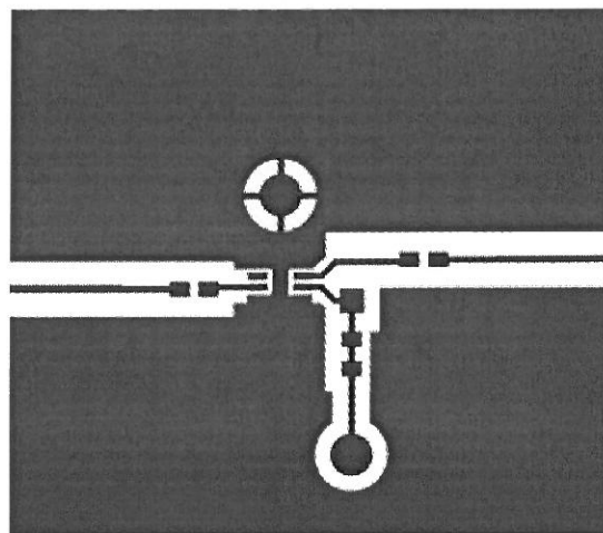
Figure 42. Component Side
