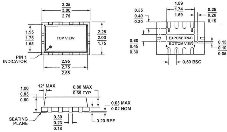
Figure 43. 8-Lead Lead Frame Chip Scale Package [LFCSP_VD] 2 mm x 3 mm Body, Very Thin, Dual Lead CP-8-1 Dimensions shown in millimeters
