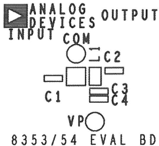
Figure 41. Silkscreen Top
