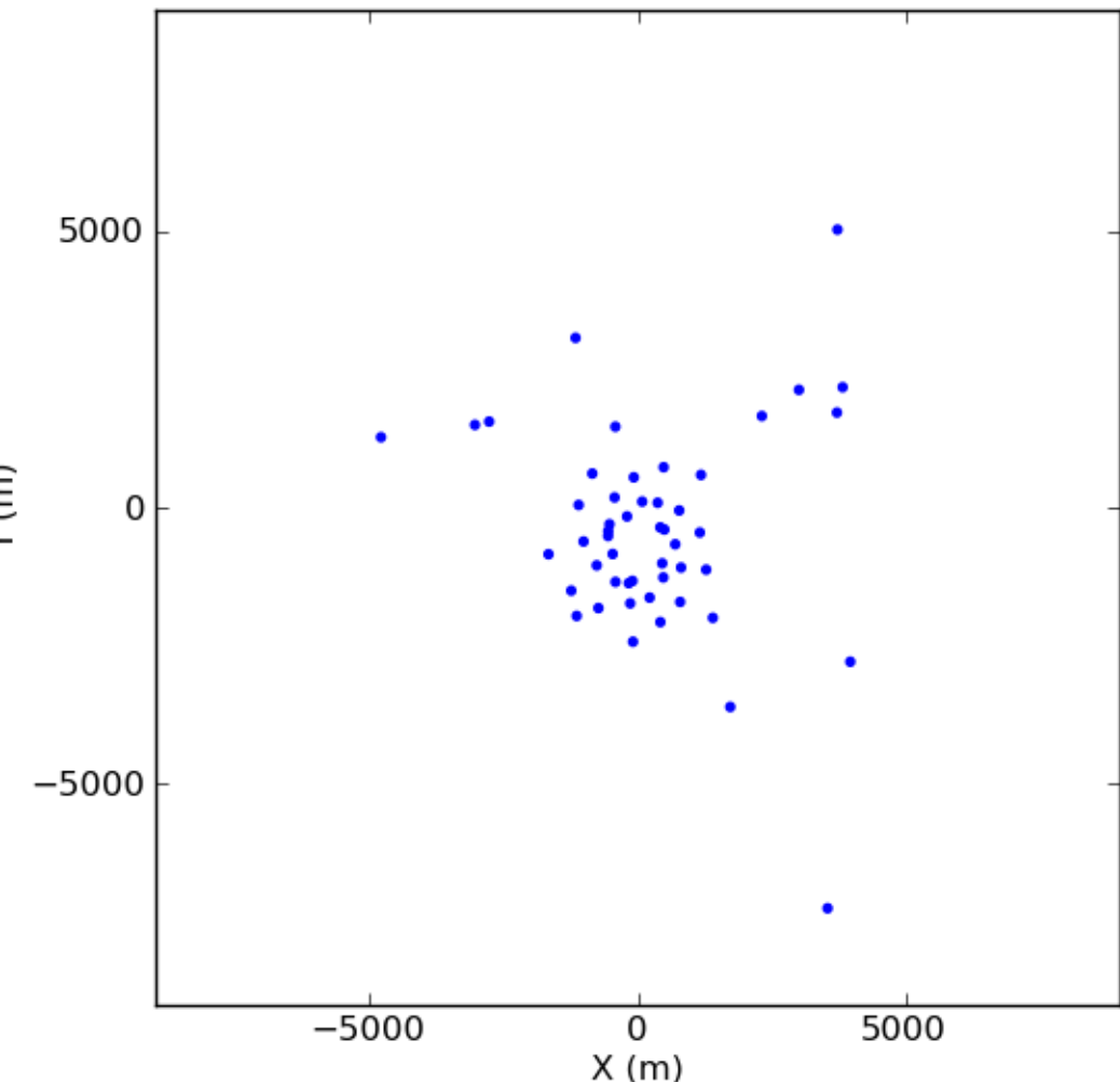
ALMA 23 (antenna size exaggerated)
