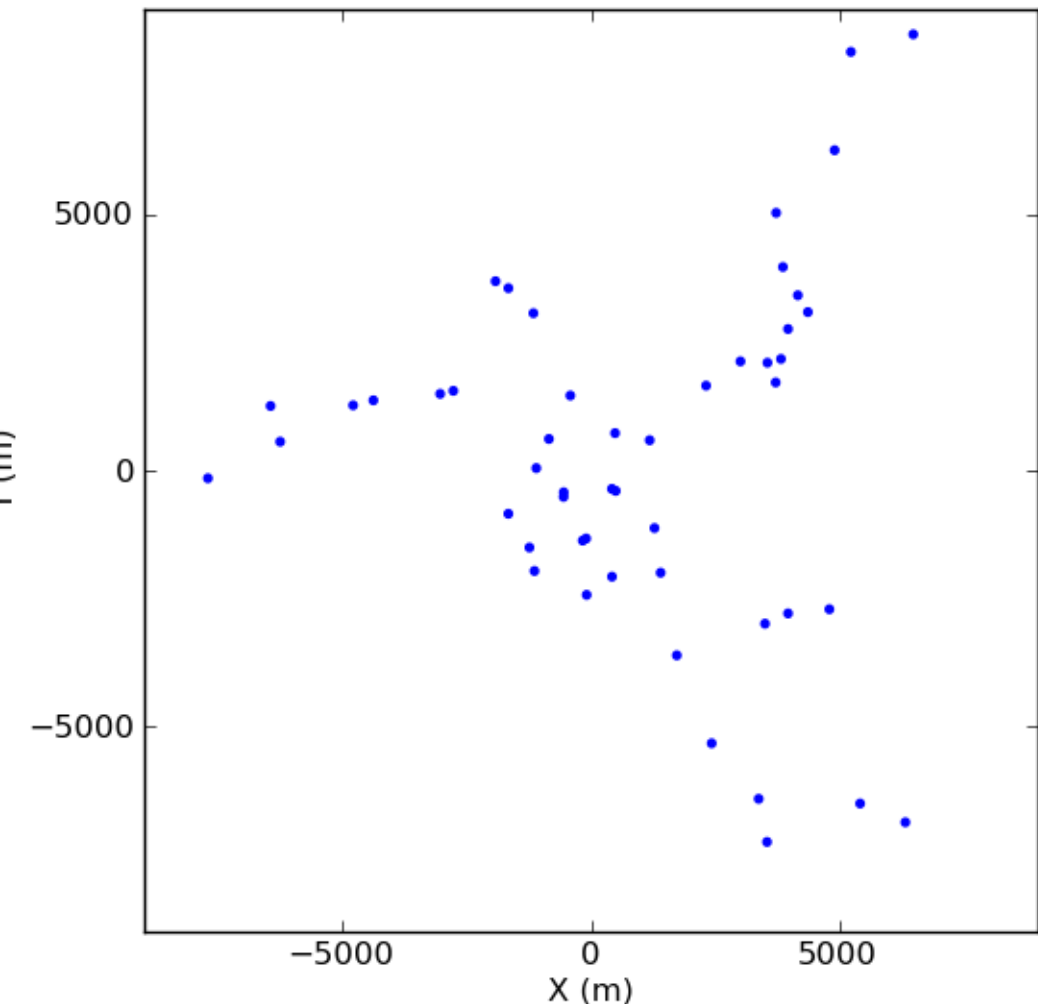
ALMA 28 (antenna size exaggerated)
