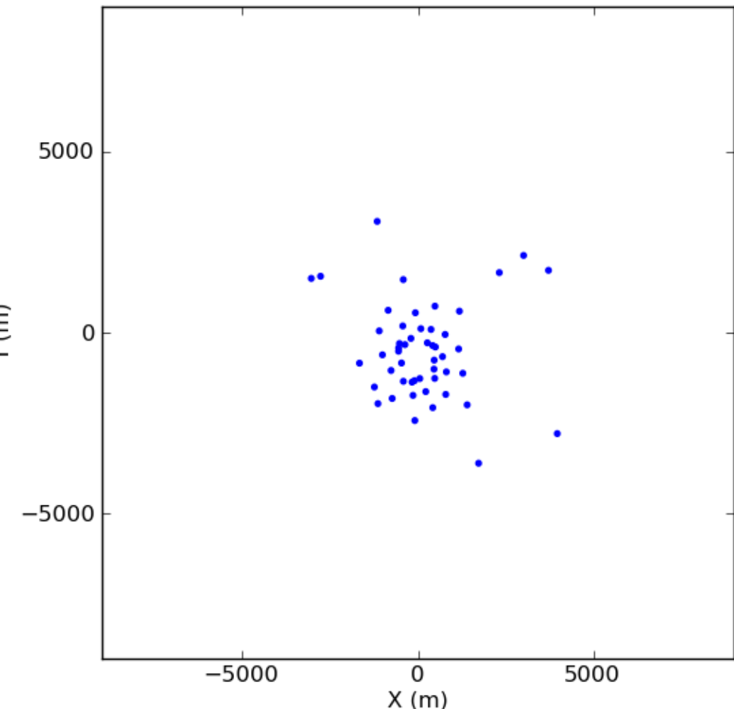
ALMA 22 (antenna size exaggerated)
