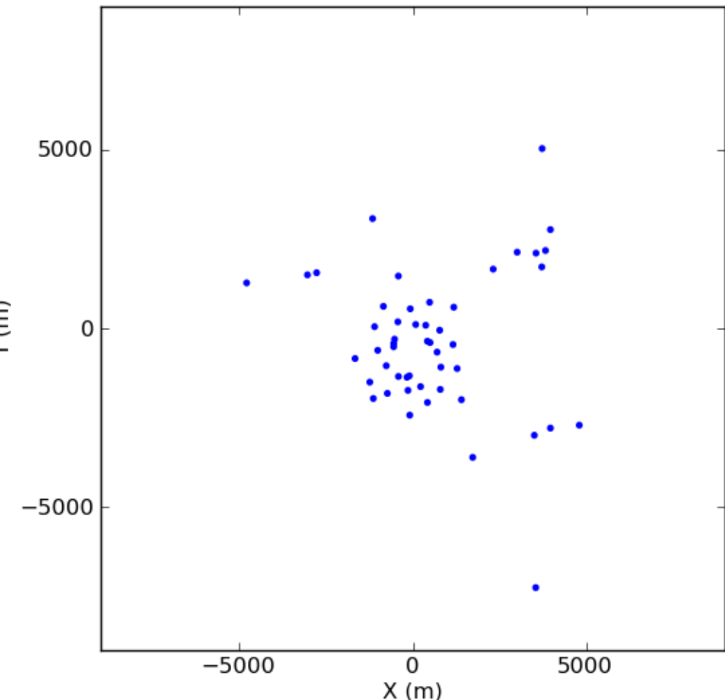
ALMA 24 (antenna size exaggerated)
