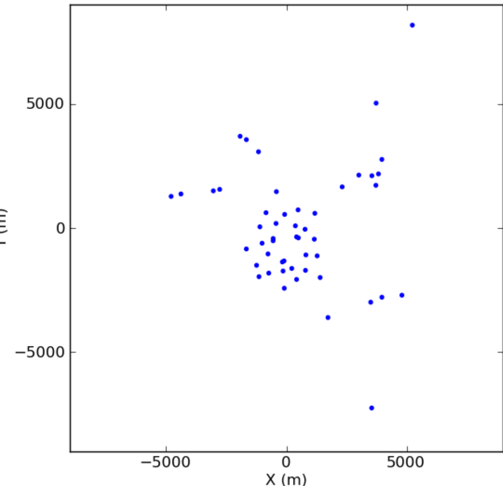
ALMA 25 (antenna size exaggerated)
