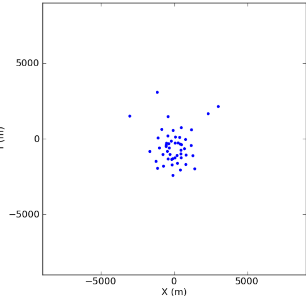
ALMA 21 (antenna size exaggerated)
