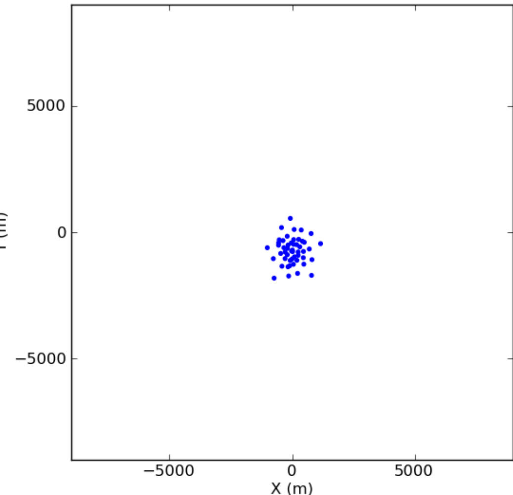
ALMA 17 (antenna size exaggerated)
