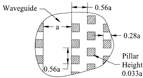
Fig. 2. Physical configuration of photonic crystal array.
