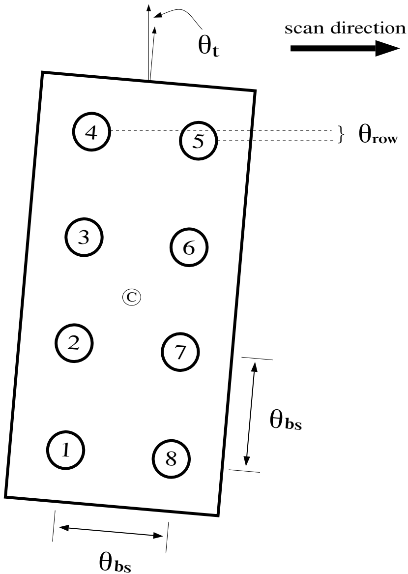
Figure 1: Beam configuration for 8-Beam receiver
