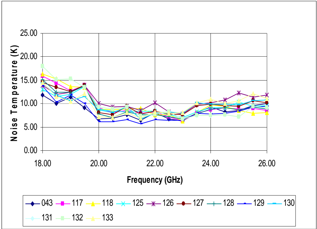
Figure 5: Measured noise for 12 of the LNAs currently built for the 7-beam KFPA. Amplifiers used in the single-beam test receiver are SN125 (LCP) and 126 (RCP).
