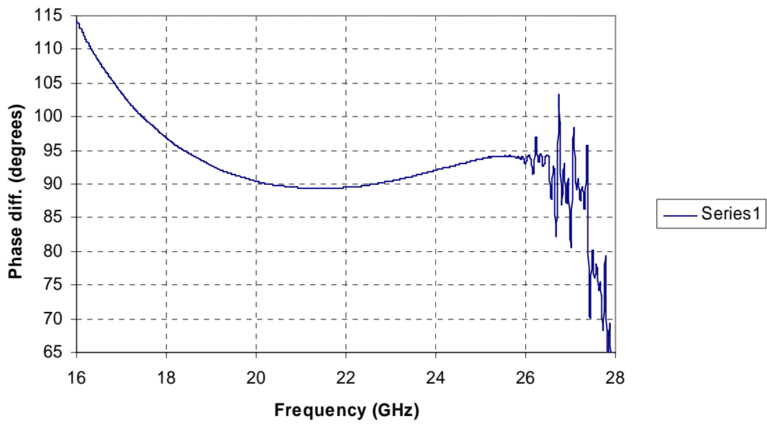
K01a; K-band phase shifter; 38 pitches
