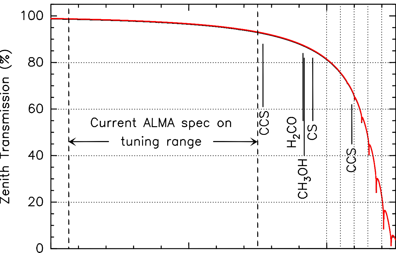
ALMA Band 1 (model: am version 5.2)
